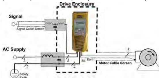
Example AC Fed Inverter shown.
